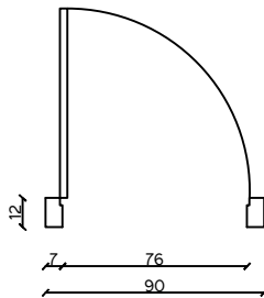
DOOR 90X210 ALL DIMENSIONS ARE IN CM.
